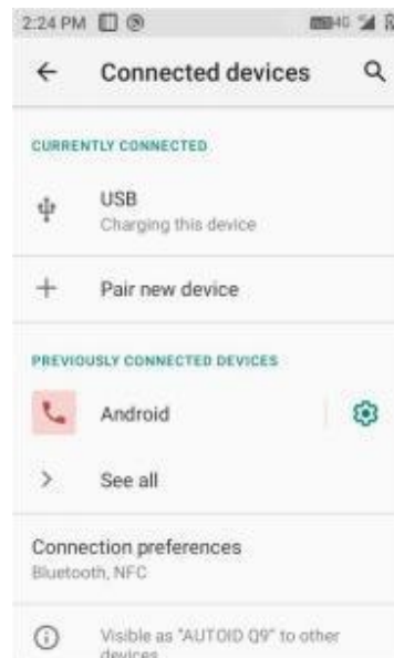
Figure 7-21 Connected Devices
