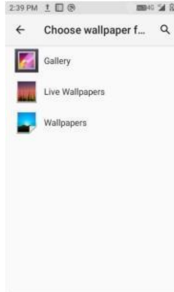
Figure 7-30 Wallpaper
