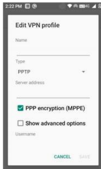
Figure 7-20 VPN Settings
