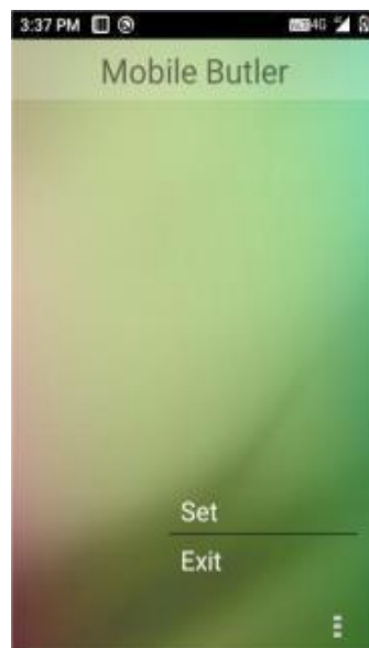
Figure 8-25 Menu Button
