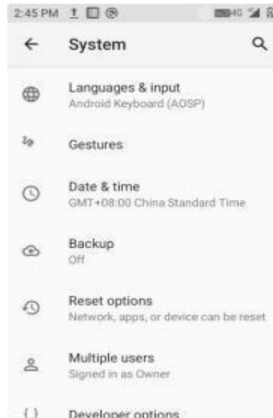
Figure 7-40 System
