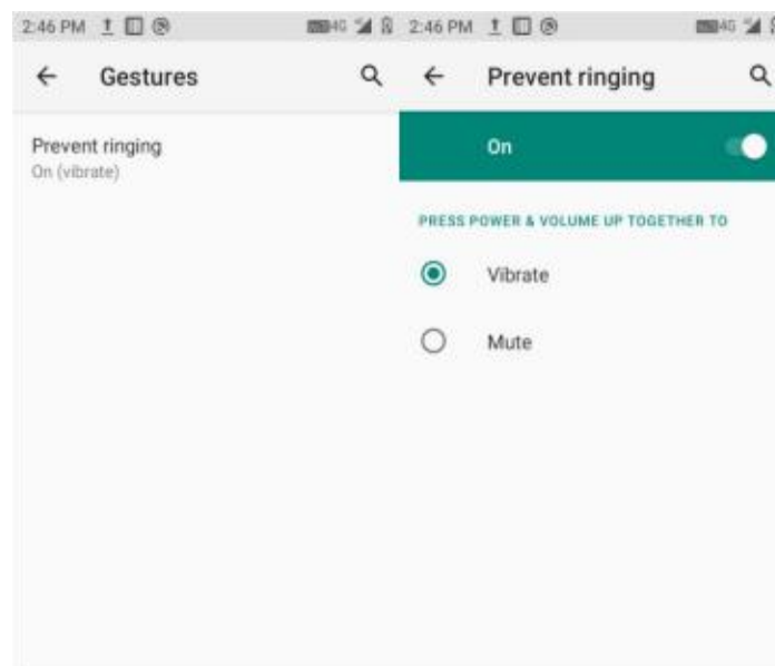
Figure 7-42 Gestures
