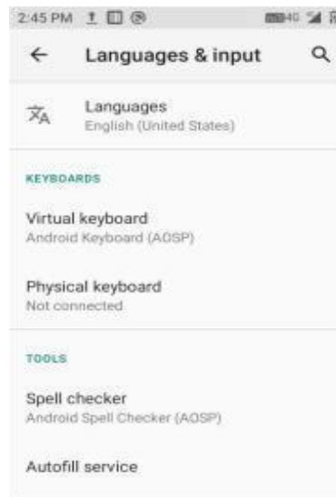
Figure 7-41 Languages & Input
