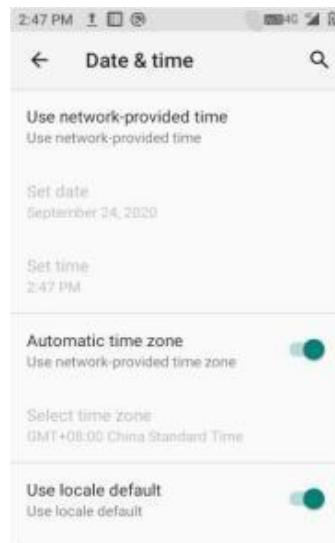
Figure 7-43 Date & Time
