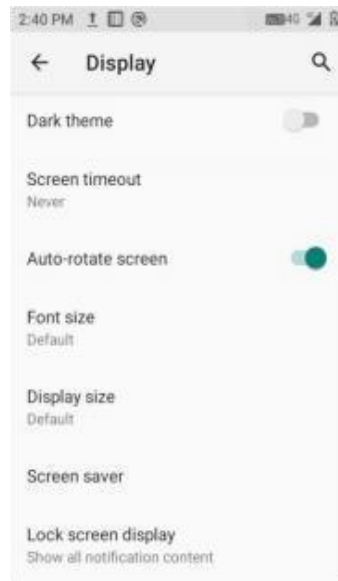
Figure 7-33 Auto Rotation
