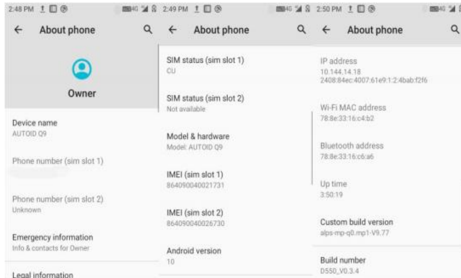
Figure 7-45 About Phone
