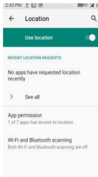
Figure 7-36 Location
