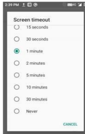
Figure 7-31 Dormancy
