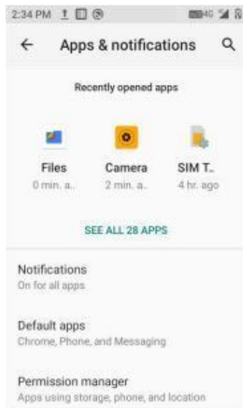
Figure 7-27 Apps & Notifications
