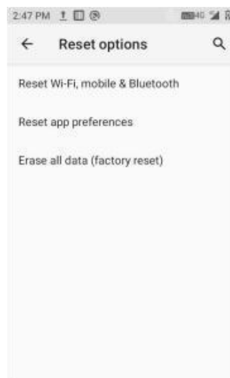
Figure 7-44 Reset options
