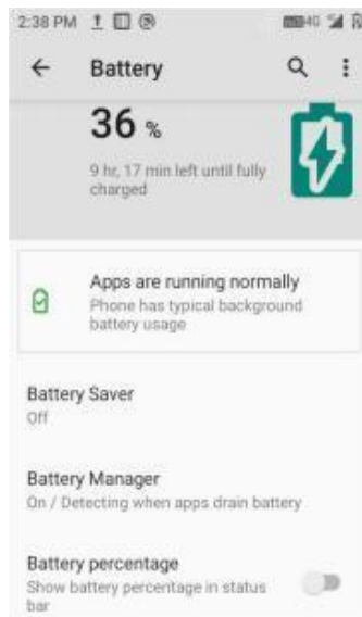
Figure 7-28 Battery
