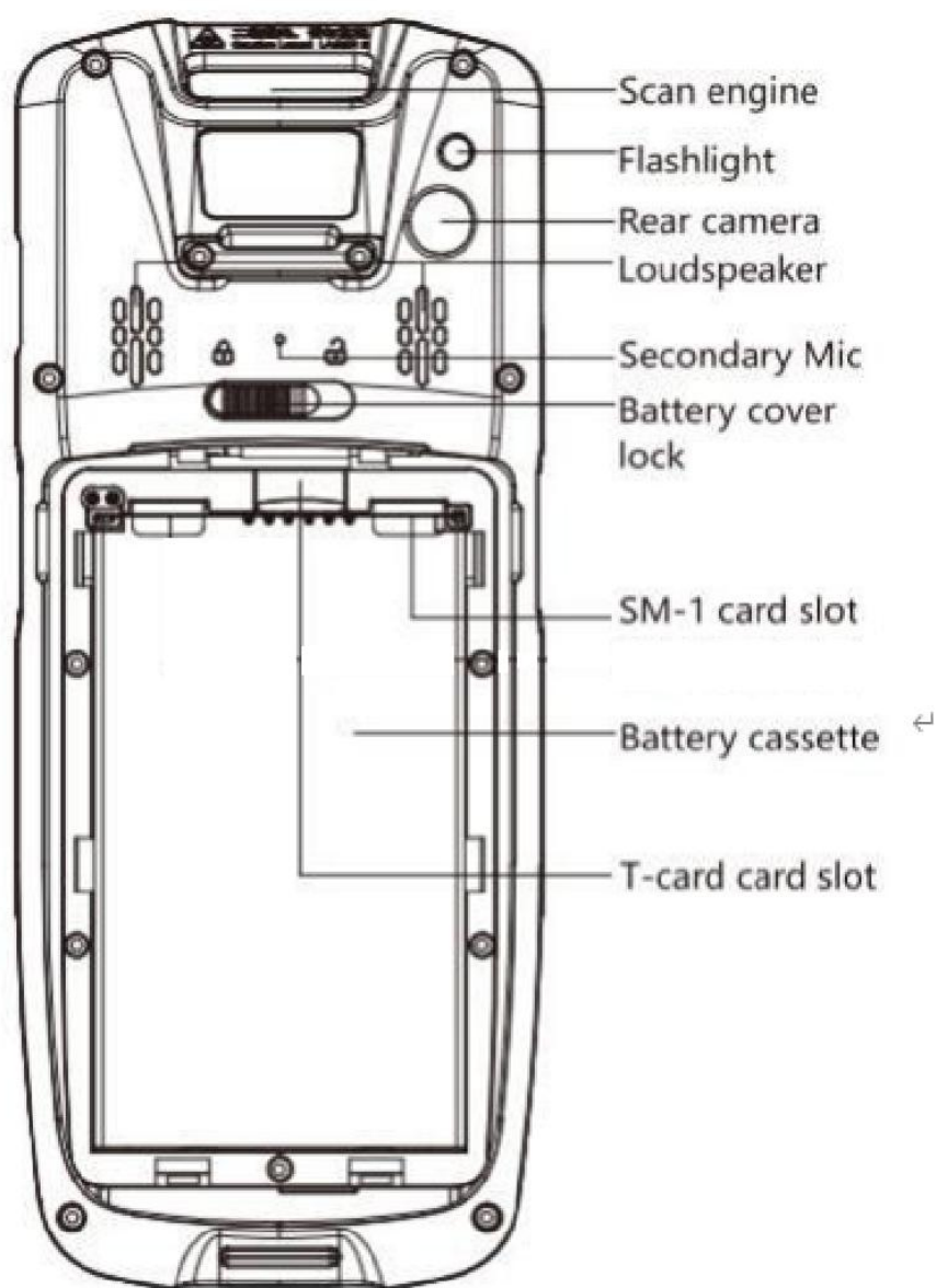
Fig 3. View for battery cassette
