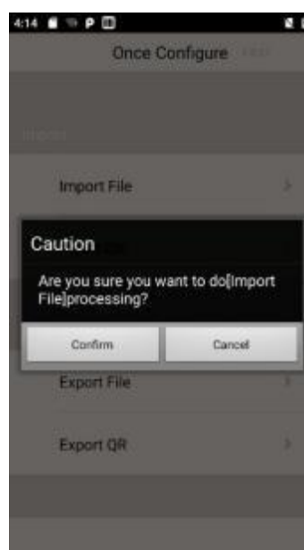
Figure 8-28 File Import
