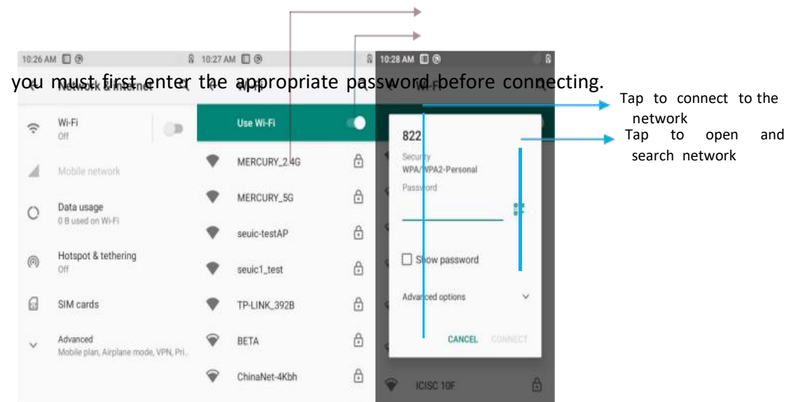
Figure 7-2 Wi-Fi menu
