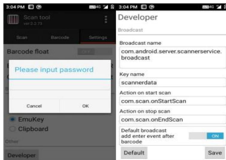
Figure 8-8 Developer Options
