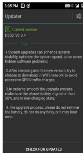
Figure 8- 10 System Update
