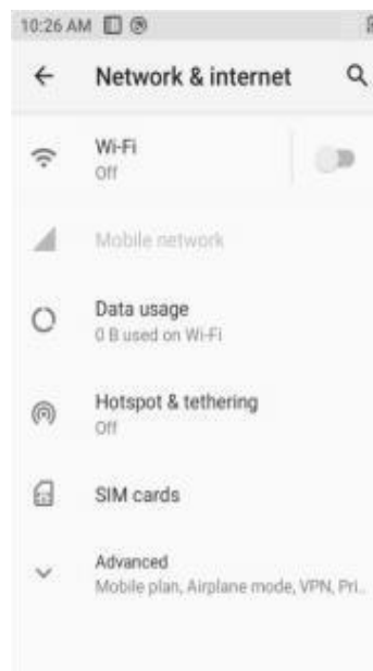
Figure 7- 1 Network & internet
