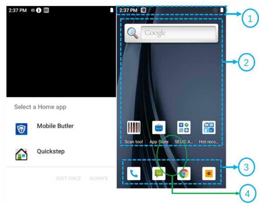
Figure 6- 1 Main Screen
