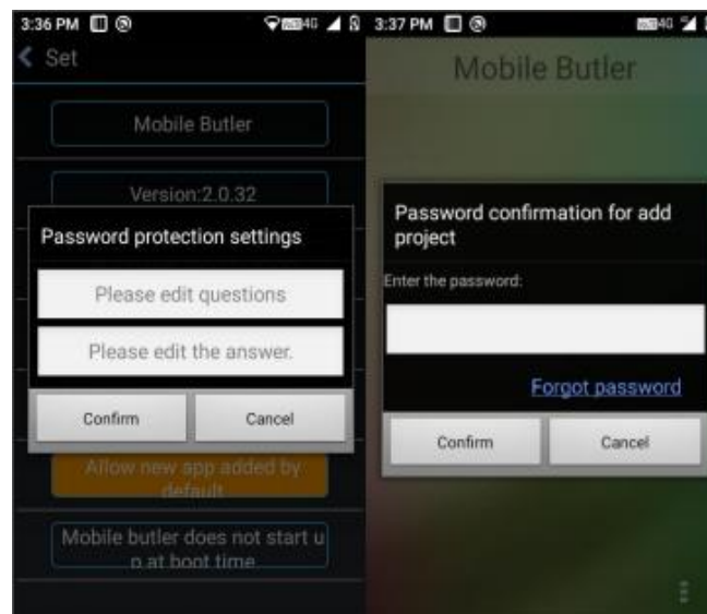
Figure 8-24 Security Settings
