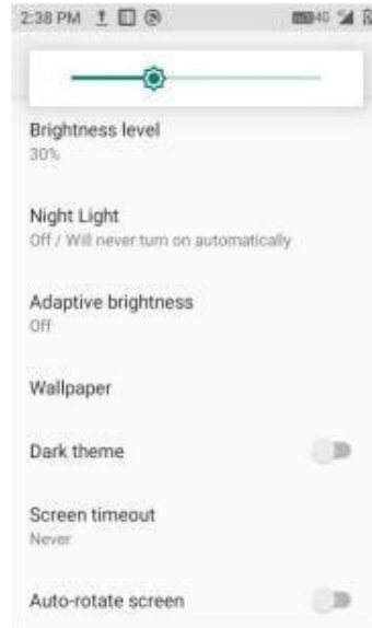
Figure 7-29 Display
