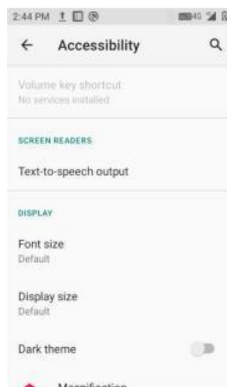
Figure 7-39 Accessibility
