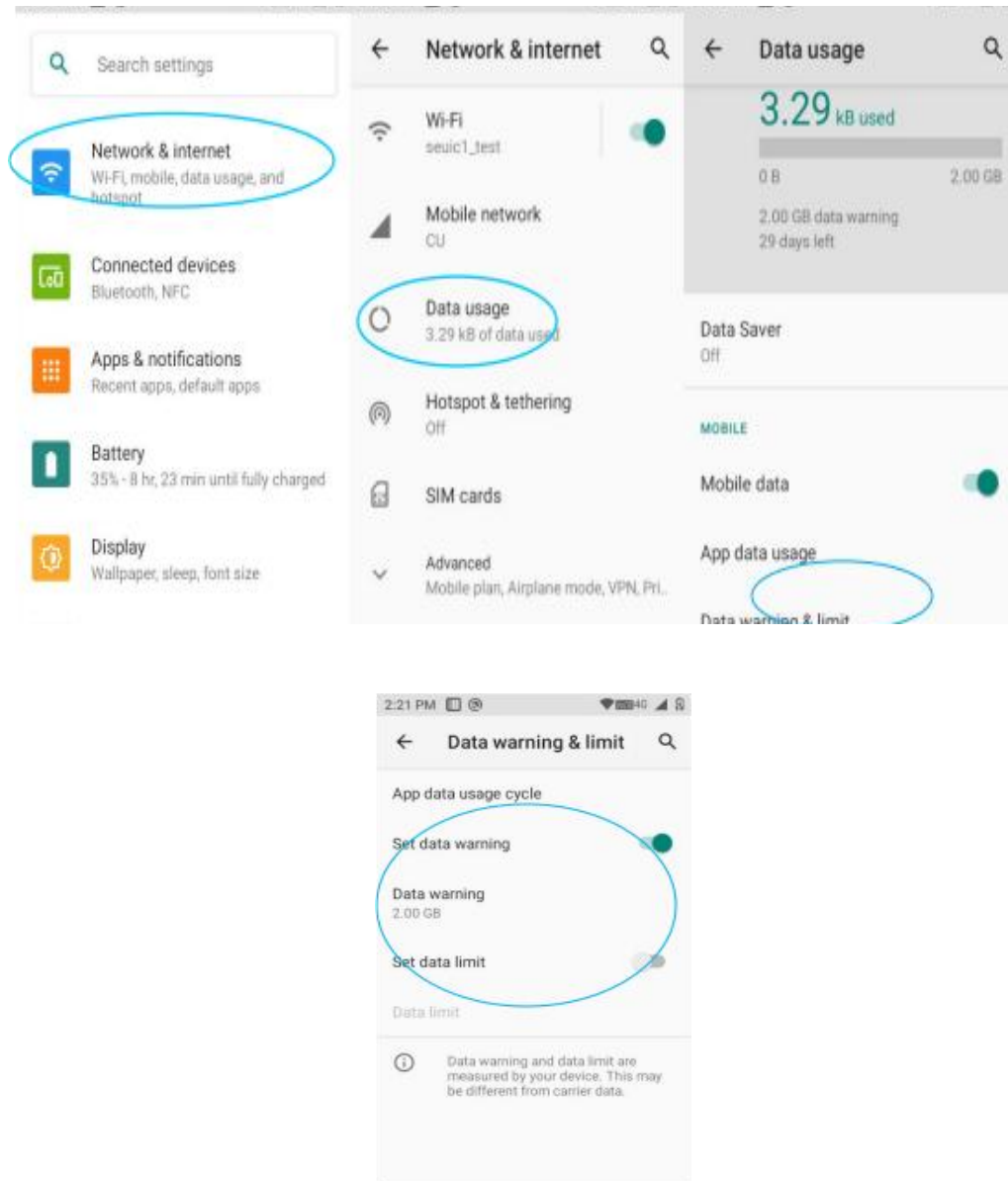
Figure 7- 17 Data usage
